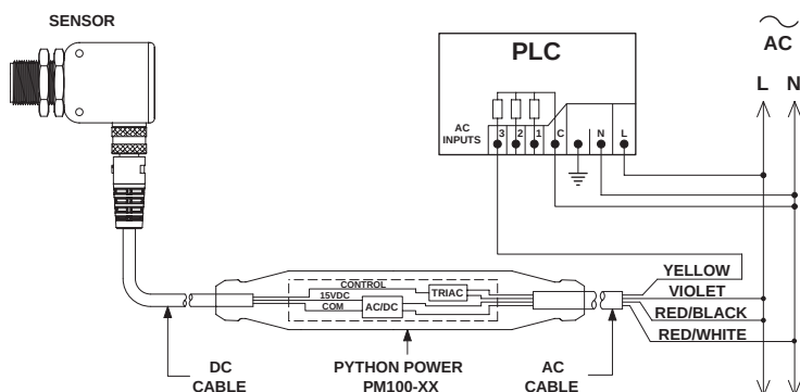
TYPICAL PLC CONNECTION
