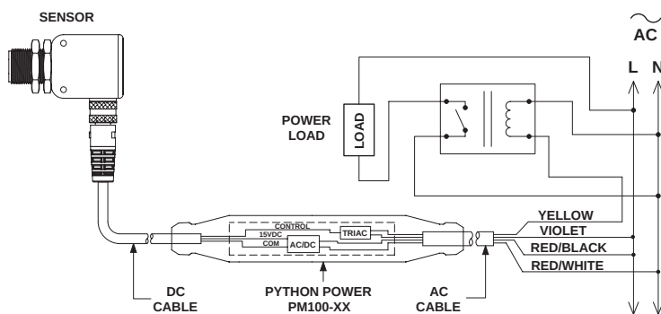
DRIVING POWER RELAY
