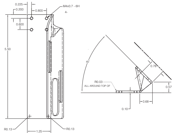
AC241 Steel/black oxide, 45° angle, label edge mounting bracket used with SUPERPROX SM6X7A-A08-01FP or SM6X7A-A08-11FP flat-profile label sensors
